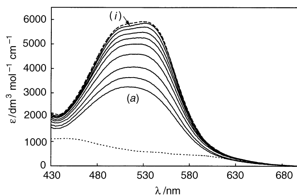
Fig. 3 Visible spectra of [LaFeL_3]^5+ in MeCN at stepwise decreasing temperature ( \Delta T = 10 K) between (a) 333 and (i) 243 K and calculated visible spectra for pure high-spin (···) and low-spin (---) [LaFeL_3]^5+ . Complex concentration: 1.2 mmol dm -3
