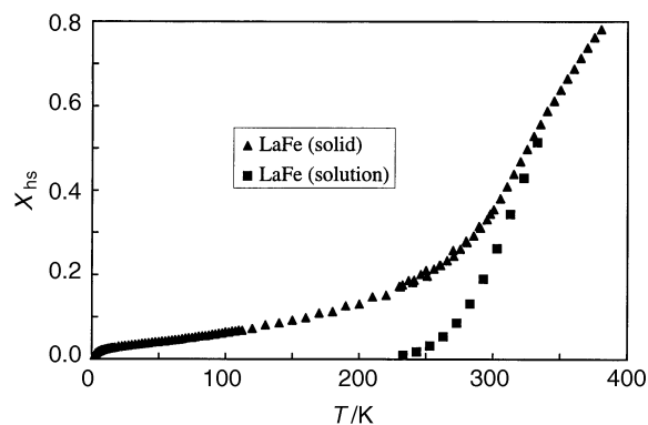
Fig. 8 Mole fraction of high-spin \text{Fe}^{\text{II}} for [\text{LaFeL}_3]^{5+} in the solid state and in solution
