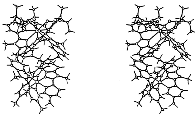
Fig. 7 An ORTEP stereoview 55 of the cation [\text{LaFeL}_3]^{5+} perpendicular to the pseudo- C_3 axis
