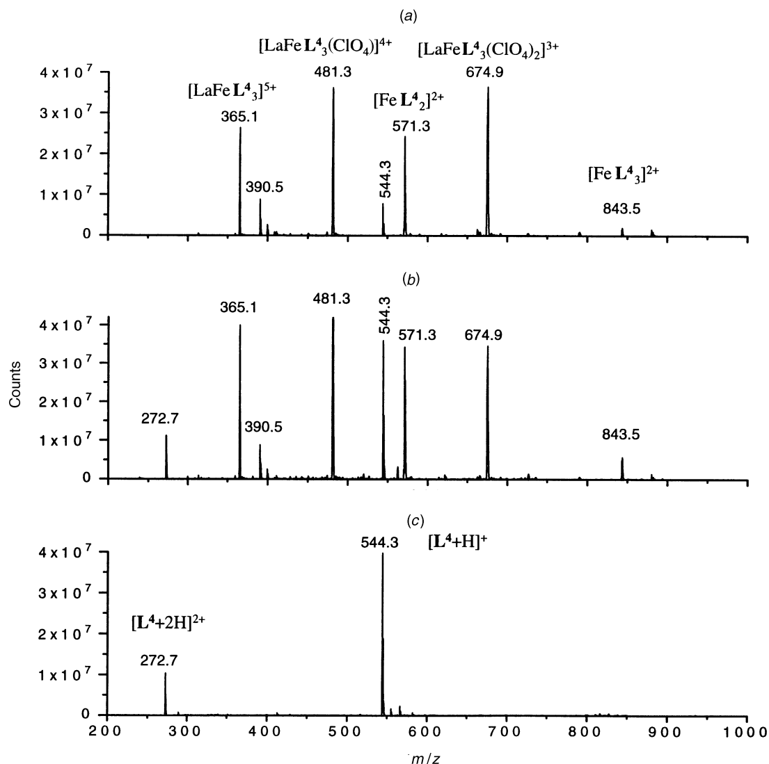
Fig. 1 Electrospray mass spectra of [\text{LaFeL}_4\text{L}_3]^{5+} in acetonitrile for total ligand concentrations of (a) 5 \times 10^{-4} , (b) 5 \times 10^{-5} and (c) 5 \times 10^{-6} \text{ mol dm}^{-3}
