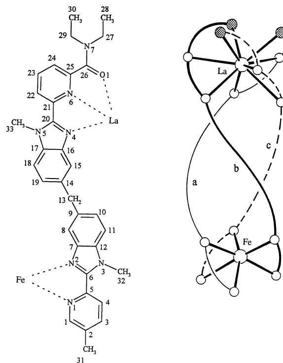
Fig. 6 Atomic numbering scheme for [\text{LaFeL}_3]^{5+} in complex 11
